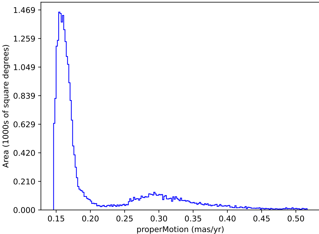
uniform_u_expt38_nscale1.1v3.4_10yrs : properMotion
