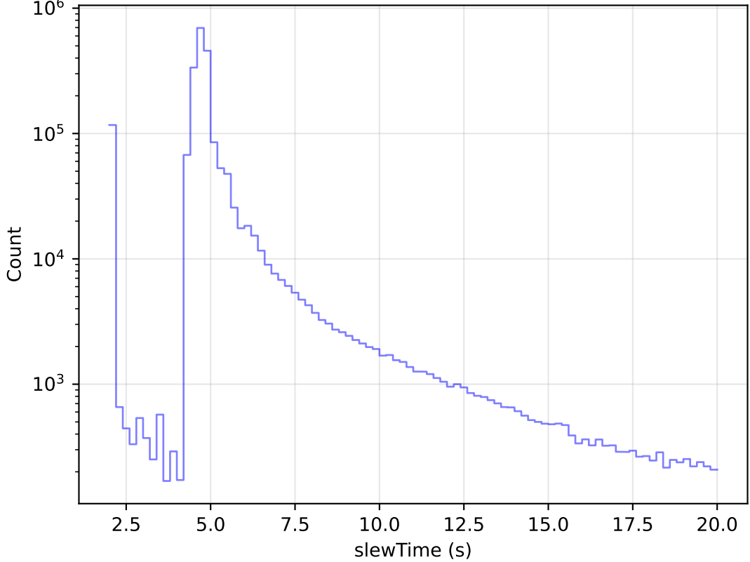
uniform_u_expt38_nscale1.1v3.4_10yrs All visits: Zoom Slew Time Histogram
