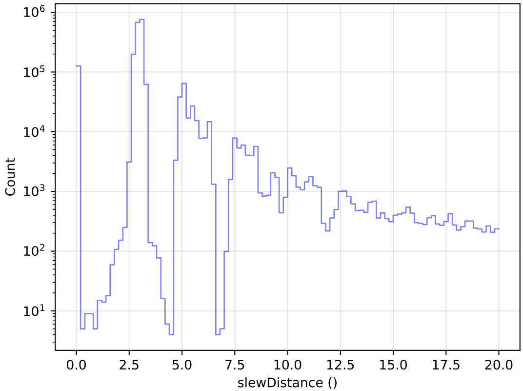
uniform_u_expt38_nscale1.1v3.4_10yrs All visits: Zoom Slew Distance Histogram
