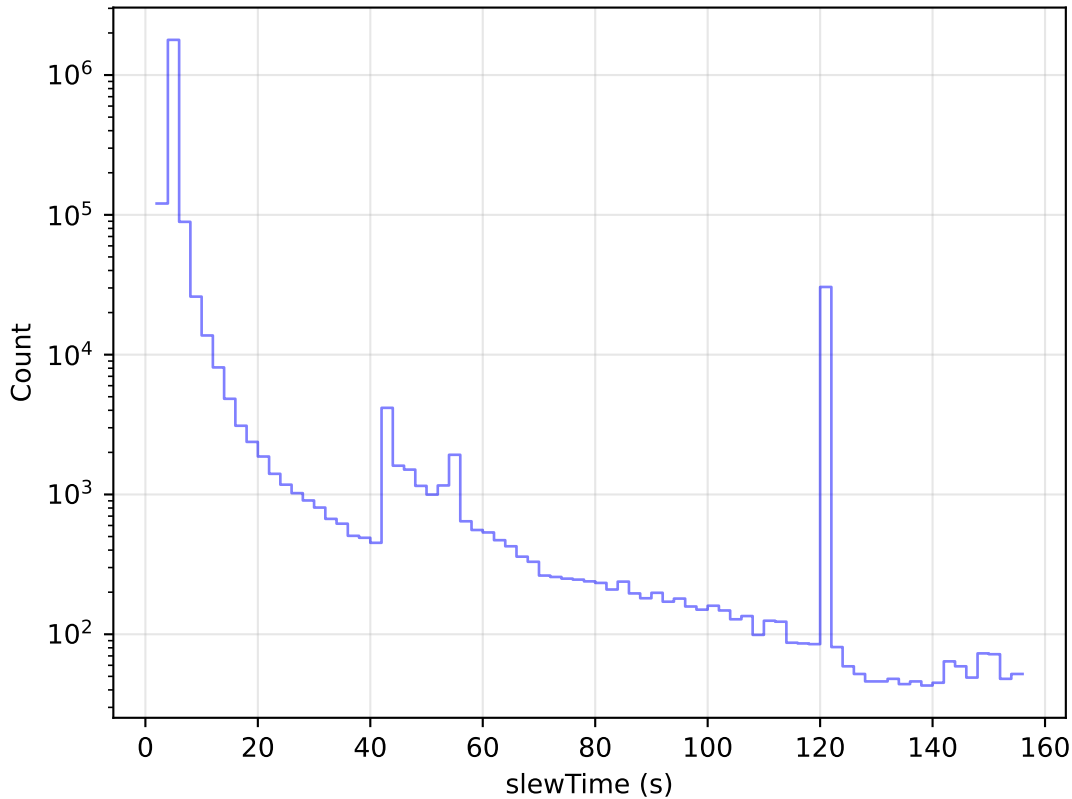
uniform_u_expt38_nscale1.1v3.4_10yrs All visits: Slew Time Histogram
