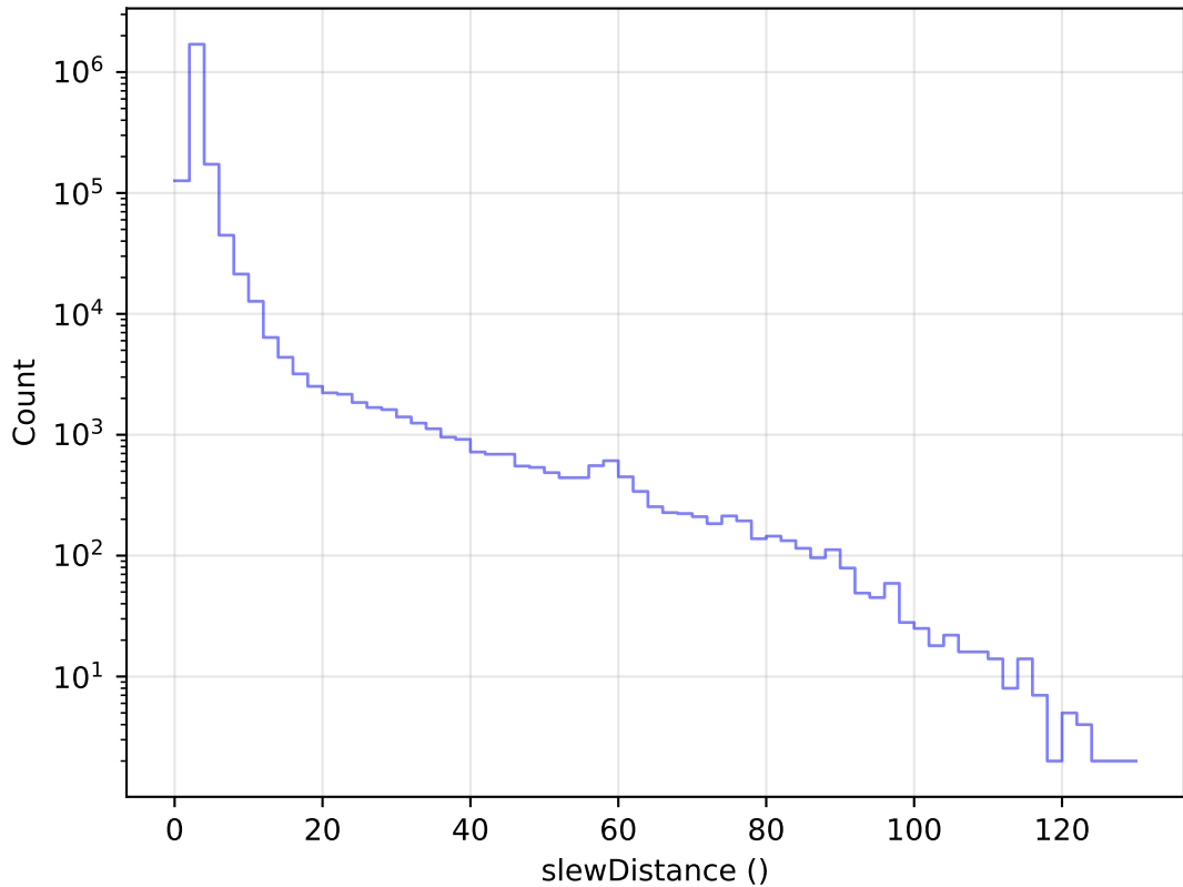
uniform_u_expt38_nscale1.1v3.4_10yrs All visits: Slew Distance Histogram
