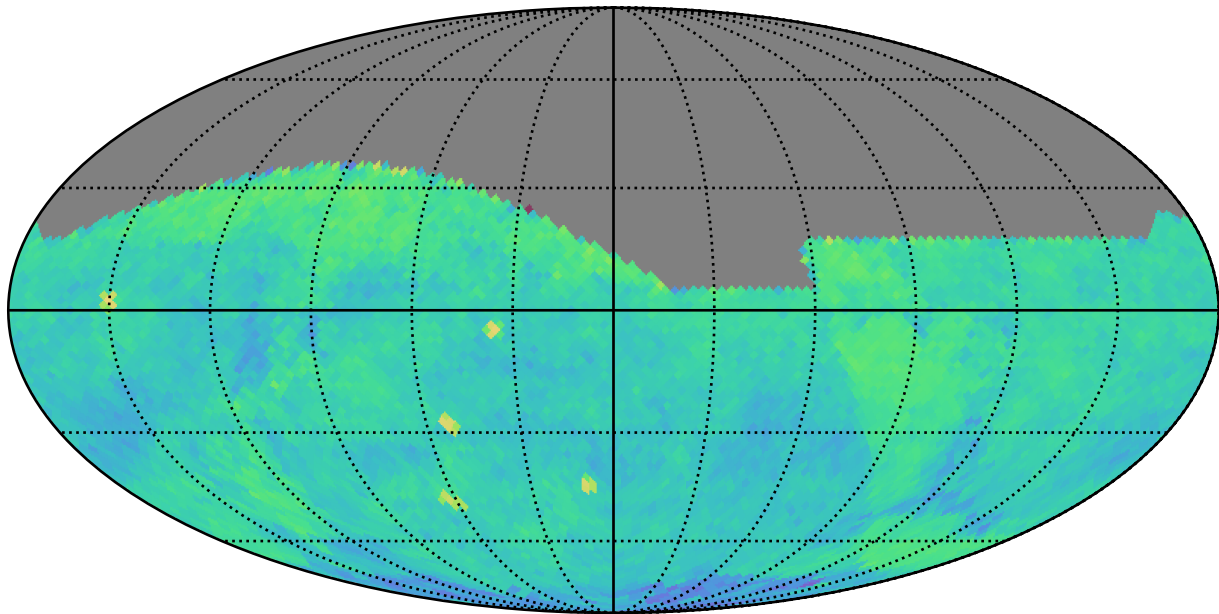
uniform_u_expt38_nscale1.1v3.4_10yrs (g or r or i): PairFraction
