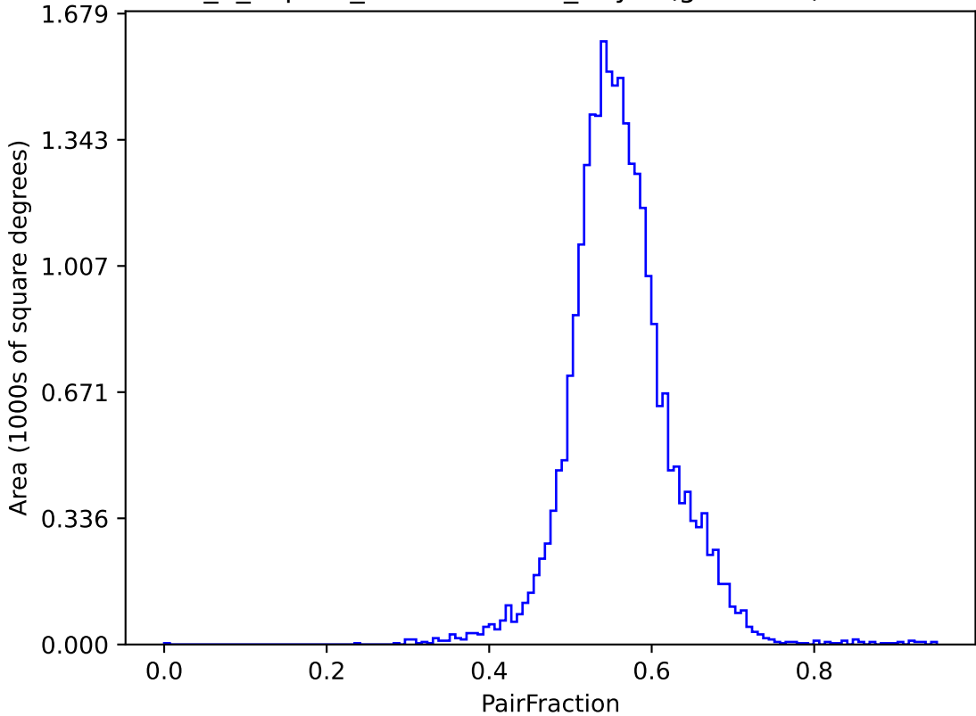
uniform_u_expt38_nscale1.1v3.4_10yrs (g or r or i): PairFraction
