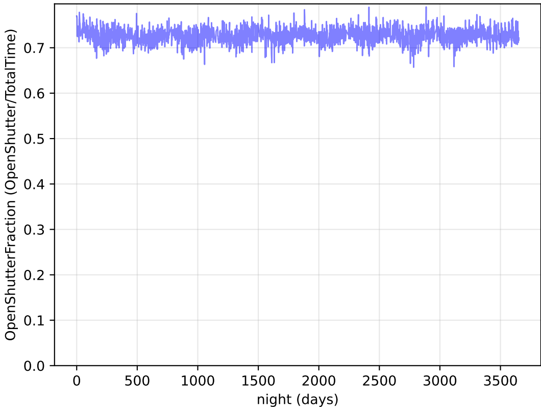
uniform_u_expt38_nscale1.1v3.4_10yrs : OpenShutterFraction
