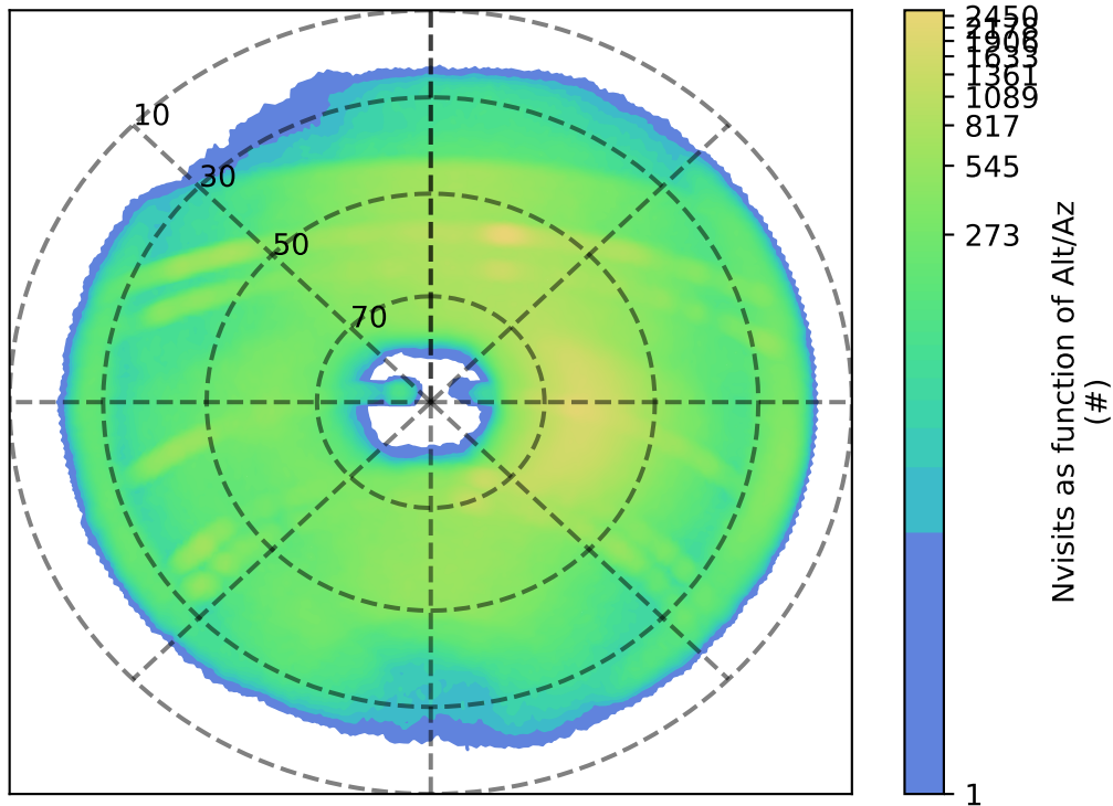
uniform_u_expt38_nscale1.1v3.4_10yrs z: Nvisits as function of Alt/Az
