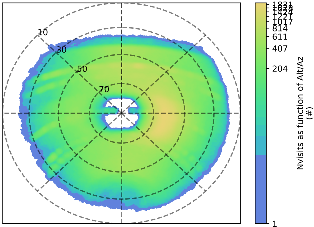
uniform_u_expt38_nscale1.1v3.4_10yrs y: Nvisits as function of Alt/Az
