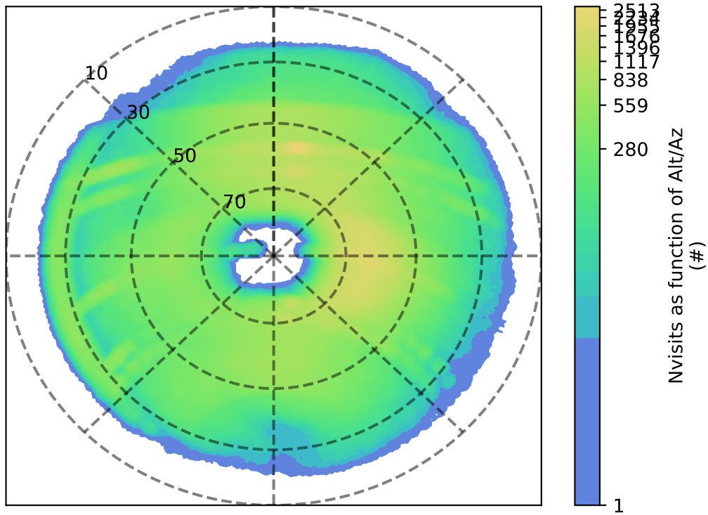
uniform_u_expt38_nscale1.1v3.4_10yrs r: Nvisits as function of Alt/Az
