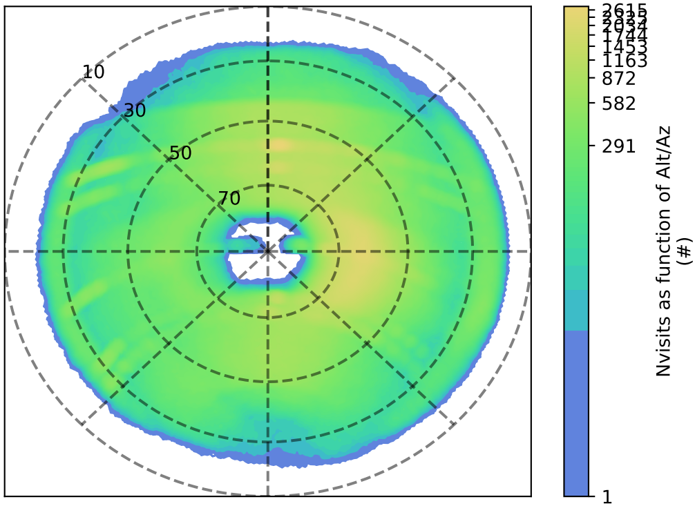
uniform_u_expt38_nscale1.1v3.4_10yrs i: Nvisits as function of Alt/Az
