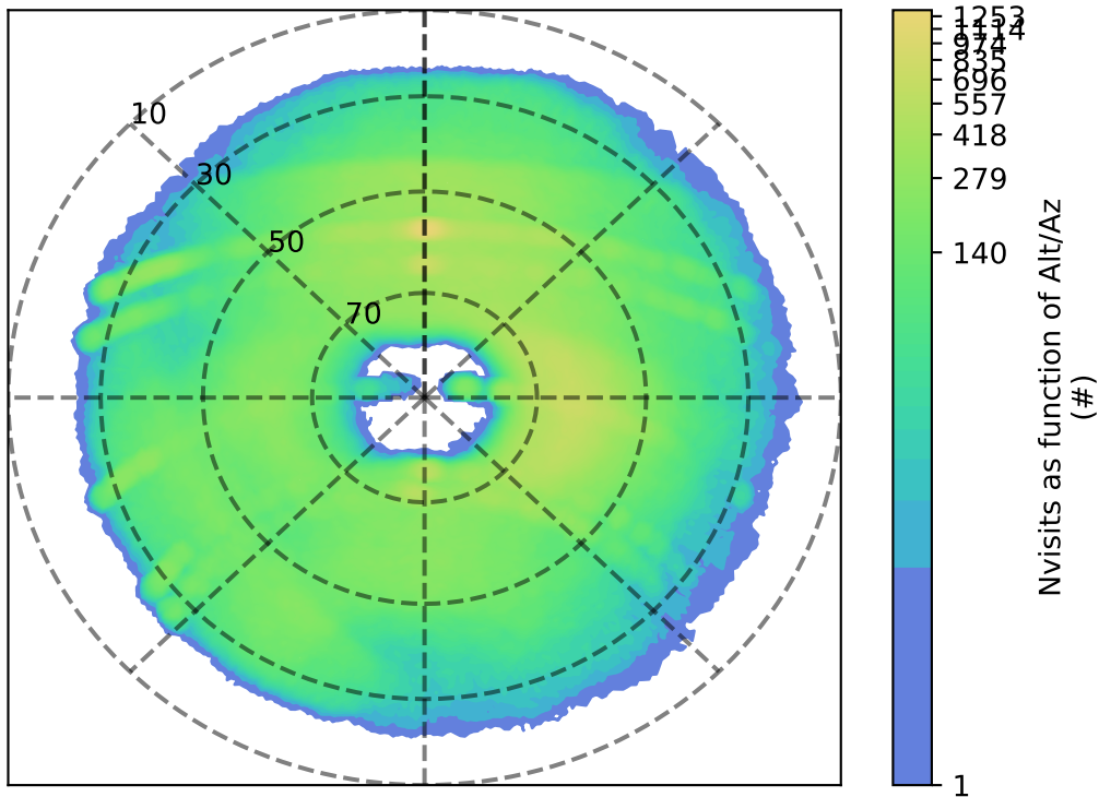
uniform_u_expt38_nscale1.1v3.4_10yrs g: Nvisits as function of Alt/Az
