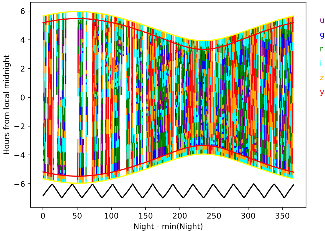
uniform_u_expt38_nscale1.1v3.4_10yrs year 8-9: Hourglass
