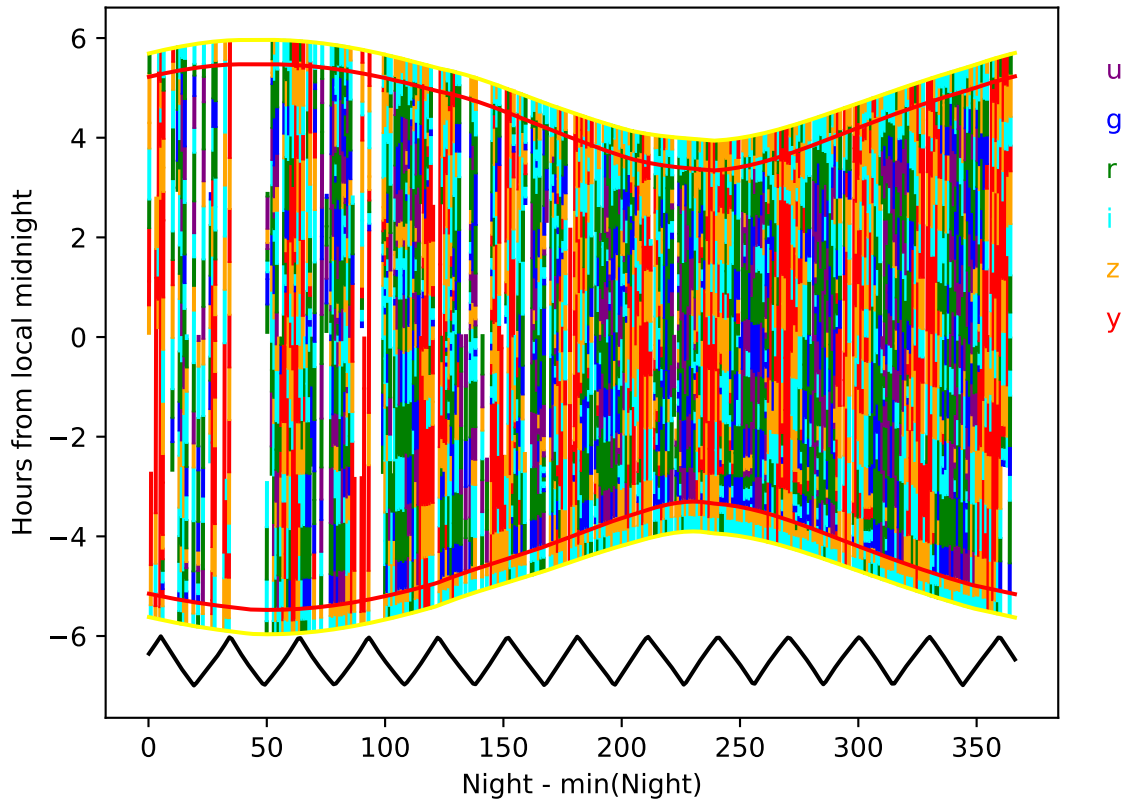
uniform_u_expt38_nscale1.1v3.4_10yrs year 6-7: Hourglass
