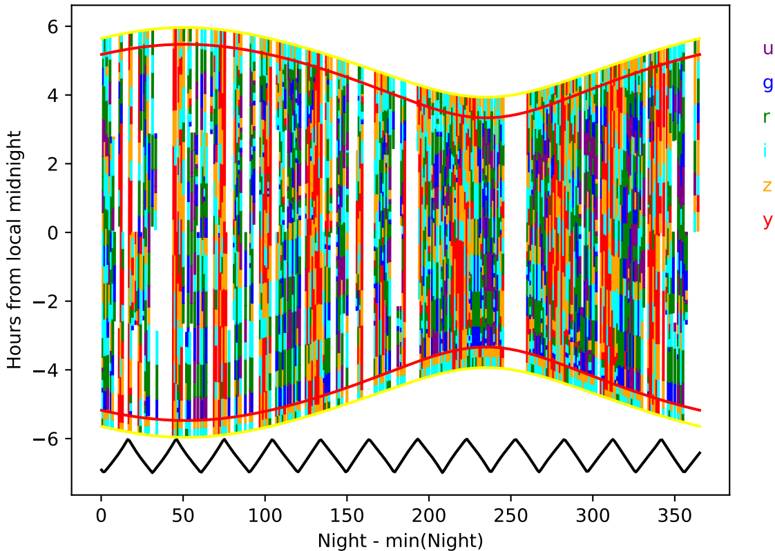
uniform_u_expt38_nscale1.1v3.4_10yrs year 5-6: Hourglass
