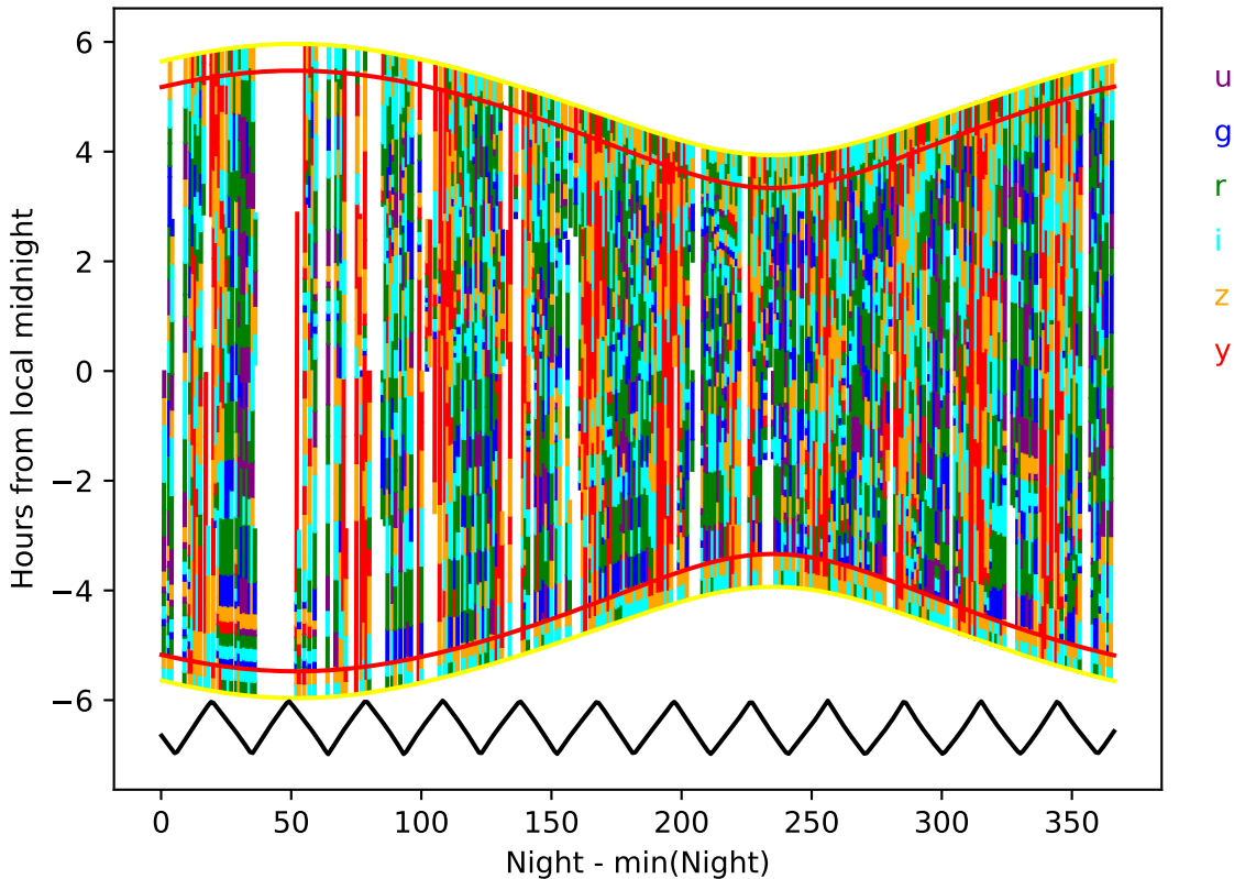
uniform_u_expt38_nscale1.1v3.4_10yrs year 2-3: Hourglass
