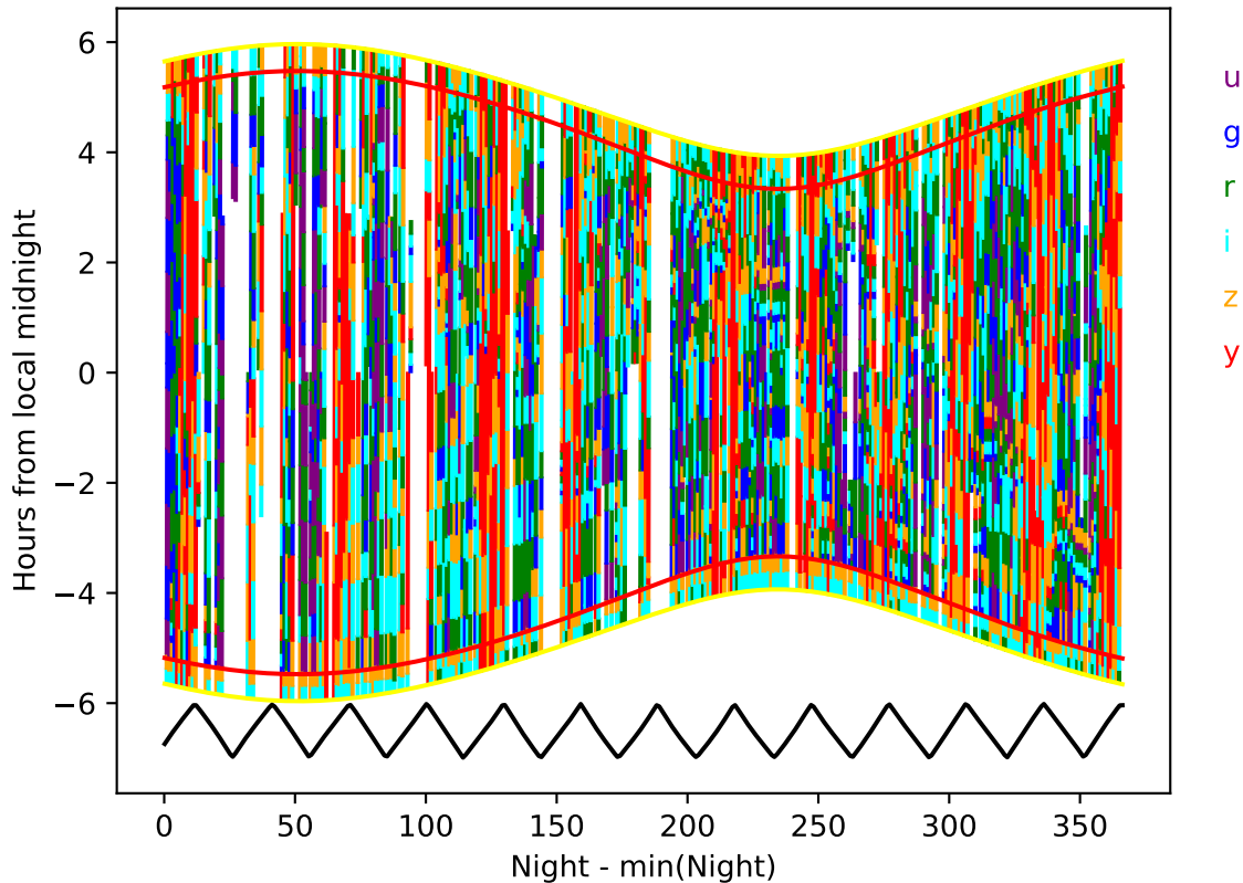
uniform_u_expt38_nscale1.1v3.4_10yrs year 0-1: Hourglass
