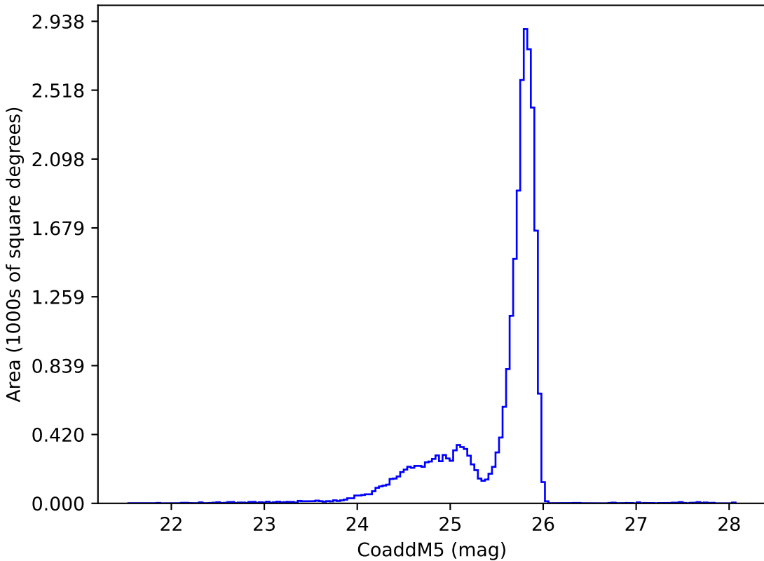
uniform_u_expt38_nscale1.1v3.4_10yrs z: CoaddM5
