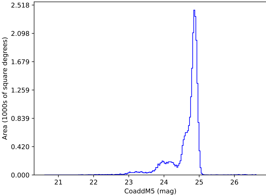
uniform_u_expt38_nscale1.1v3.4_10yrs y: CoaddM5
