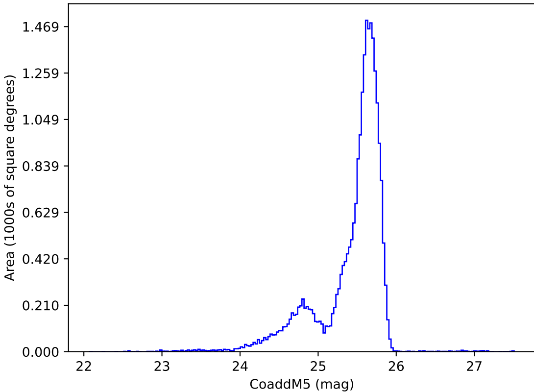
uniform_u_expt38_nscale1.1v3.4_10yrs u: CoaddM5
