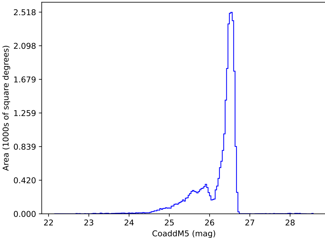
uniform_u_expt38_nscale1.1v3.4_10yrs i: CoaddM5
