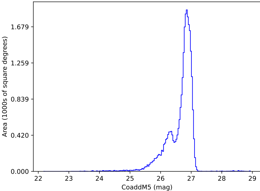
uniform_u_expt38_nscale1.1v3.4_10yrs g: CoaddM5
