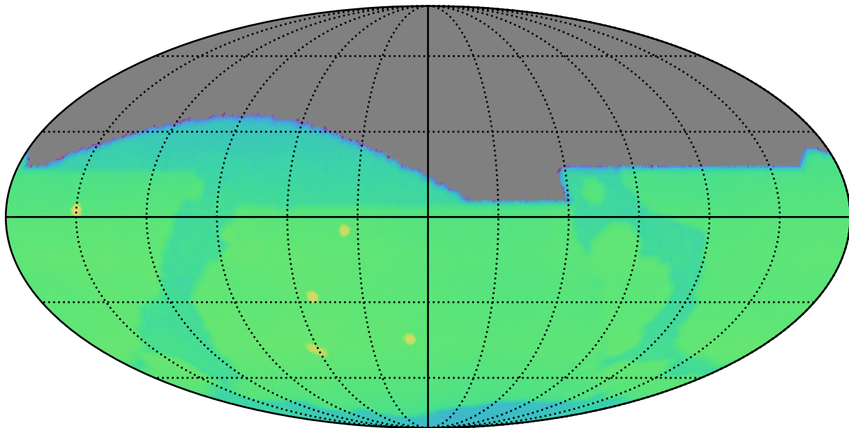
uniform_u_expt38_nscale1.1v3.4_10yrs : CoaddM5
