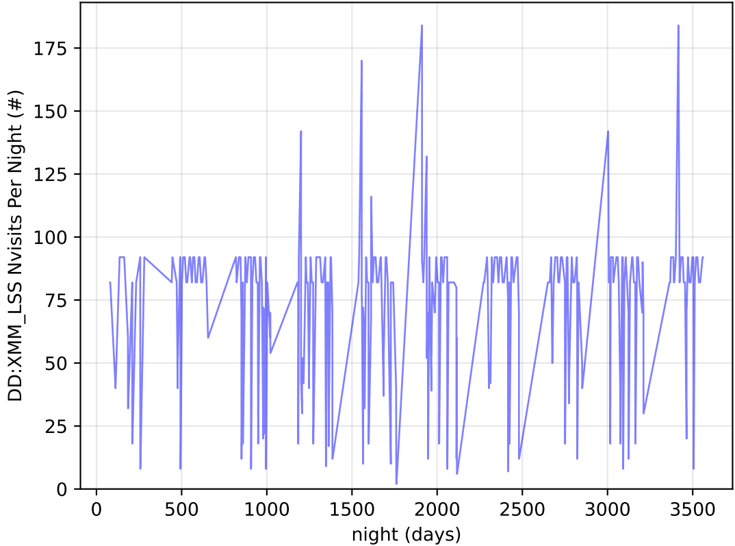
uniform_u_expt38_nscale1.1v3.4_10yrs all bands: DD:XMM_LSS Nvisits Per Night
