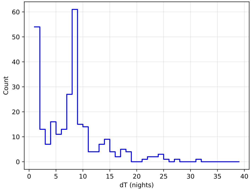
uniform_u_expt38_nscale1.1v3.4_10yrs all bands: DD:XMM_LSS Delta Nights Histogram
