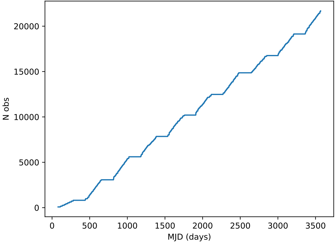
uniform_u_expt38_nscale1.1v3.4_10yrs all bands: DD:XMM_LSS Cumulative NVisits
