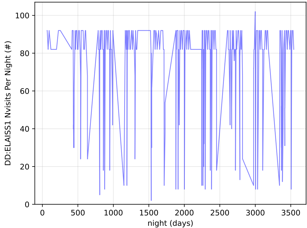
uniform_u_expt38_nscale1.1v3.4_10yrs all bands: DD:ELAISS1 Nvisits Per Night
