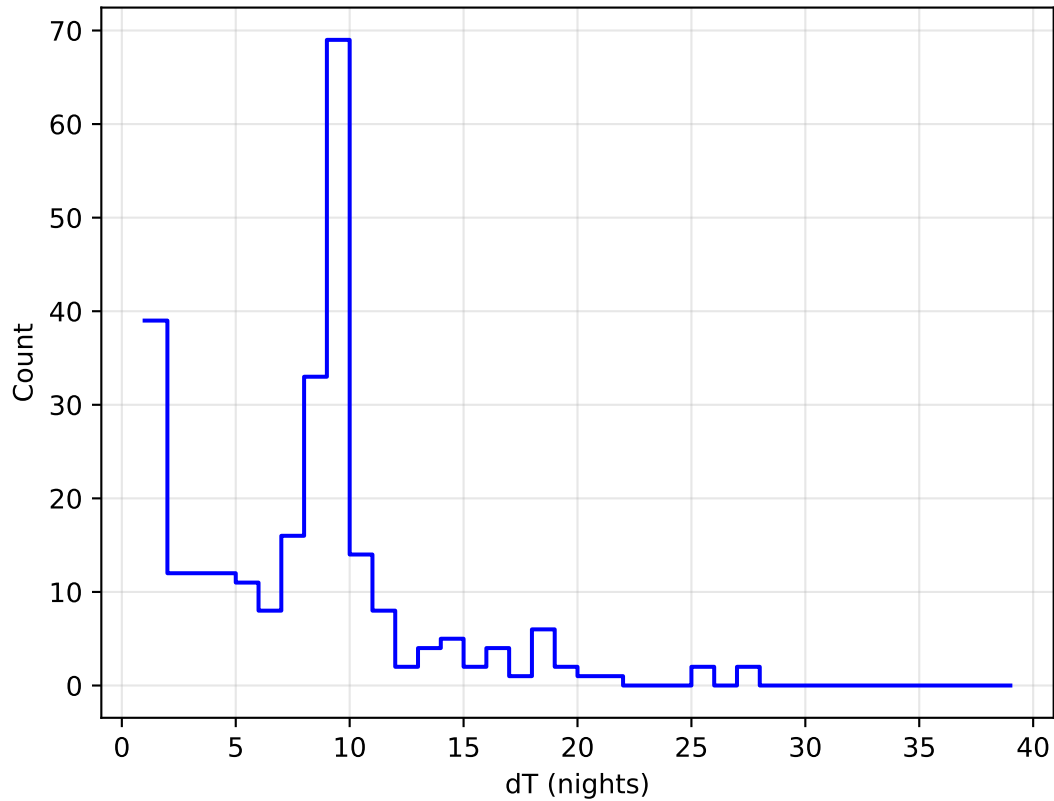
uniform_u_expt38_nscale1.1v3.4_10yrs all bands: DD:ELAISS1 Delta Nights Histogram
