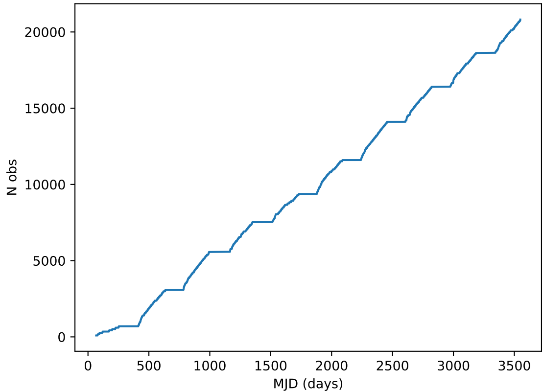
uniform_u_expt38_nscale1.1v3.4_10yrs all bands: DD:ELAISS1 Cumulative NVisits
