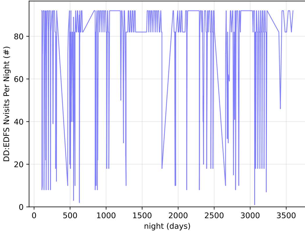
uniform_u_expt38_nscale1.1v3.4_10yrs all bands: DD:EDFS Nvisits Per Night
