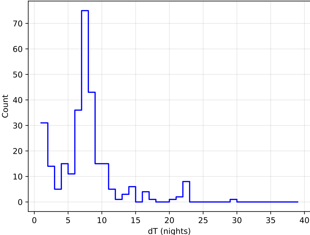
uniform_u_expt38_nscale1.1v3.4_10yrs all bands: DD:EDFS Delta Nights Histogram
