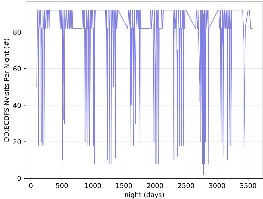
uniform_u_expt38_nscale1.1v3.4_10yrs all bands: DD:ECDFS Nvisits Per Night
