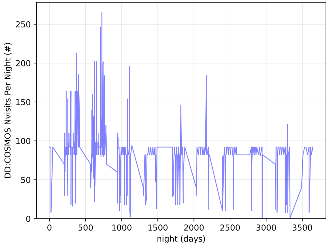
uniform_u_expt38_nscale1.1v3.4_10yrs all bands: DD: COSMOS Nvisits Per Night
