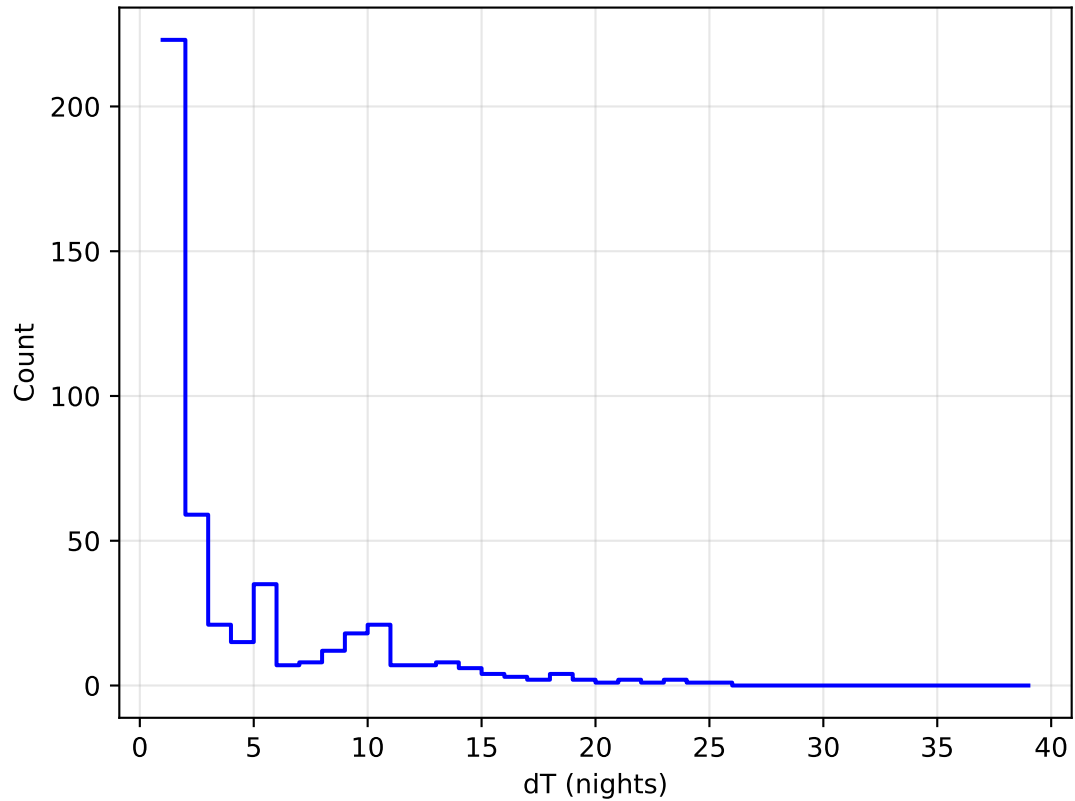
uniform_u_expt38_nscale1.1v3.4_10yrs all bands: DD:COSMOS Delta Nights Histogram
