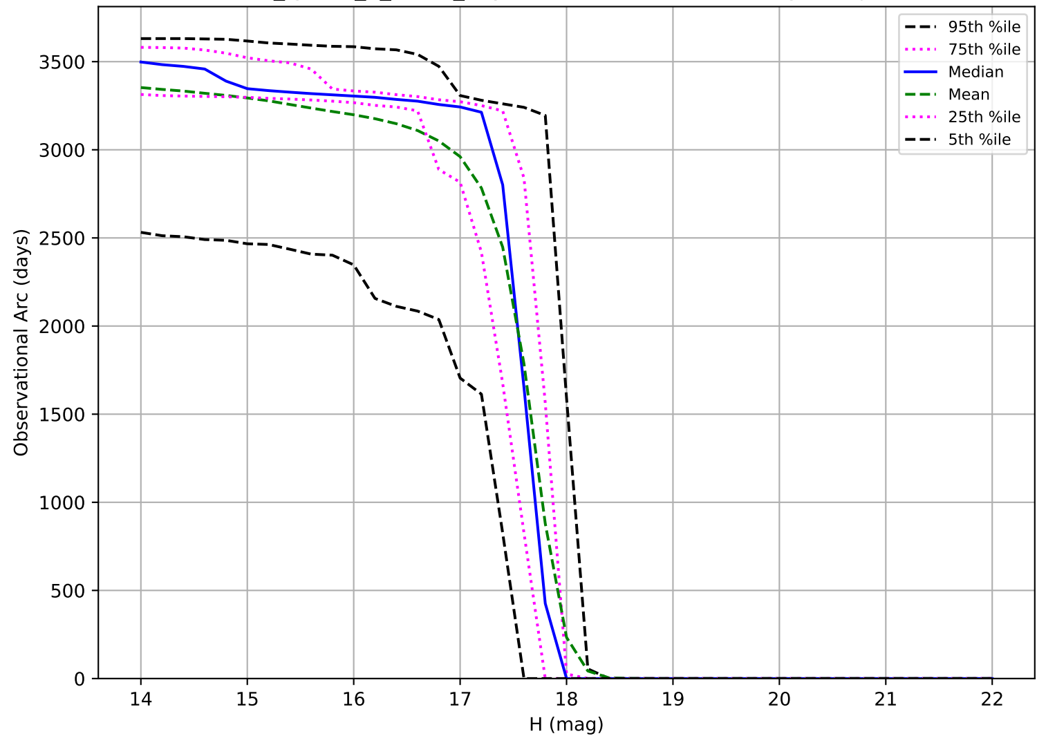
too_ignore_5_4v3.4_10yrs: Observational Arc Length Trojan
