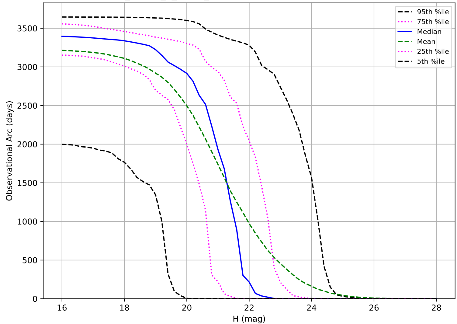
too_ignore_5_4v3.4_10yrs: Observational Arc Length PHA
