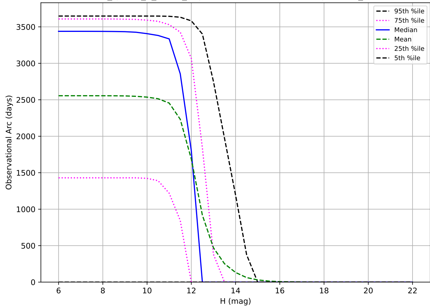
too_ignore_5_4v3.4_10yrs: Observational Arc Length OCC_r20
