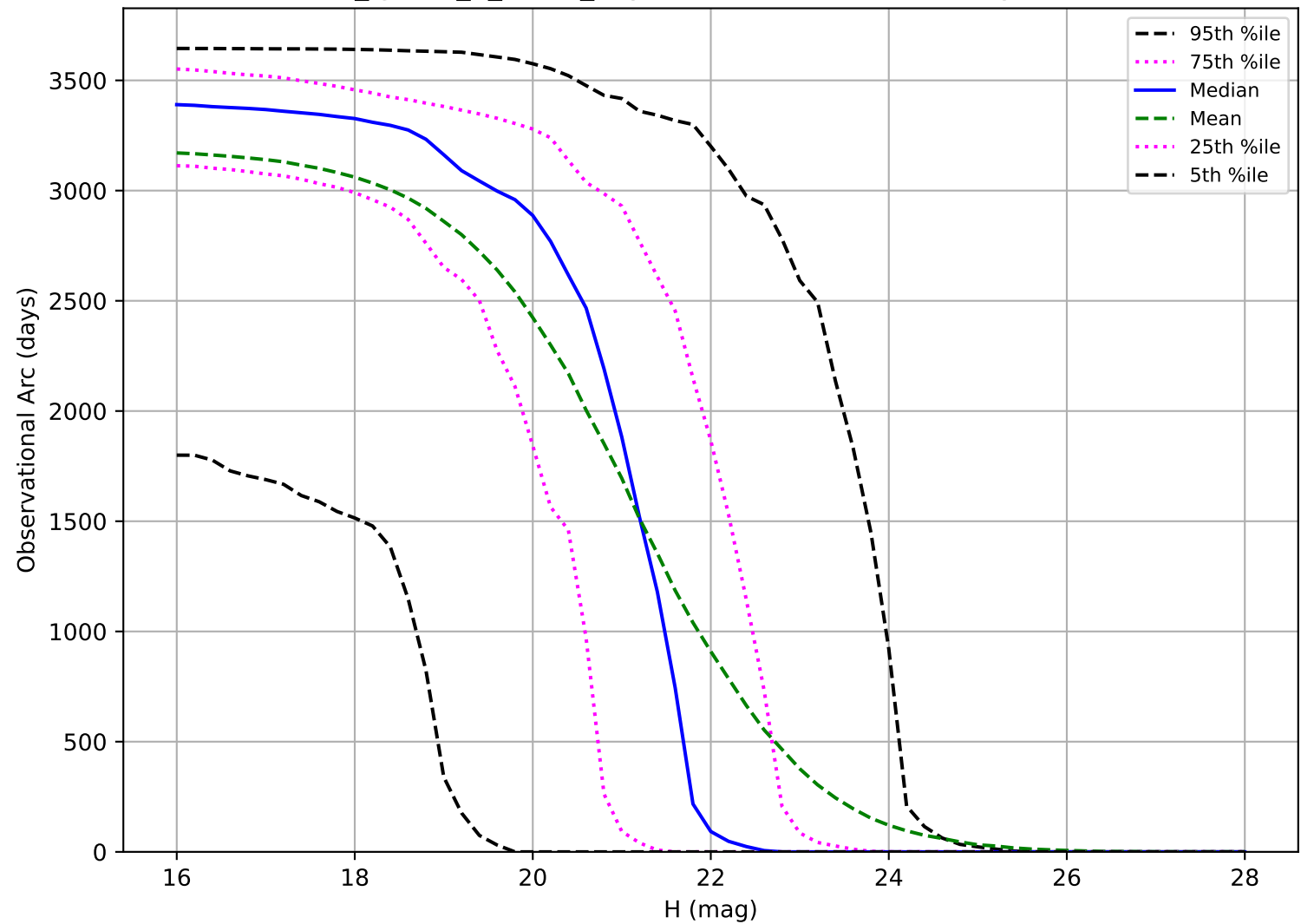
too_ignore_5_4v3.4_10yrs: Observational Arc Length NEO
