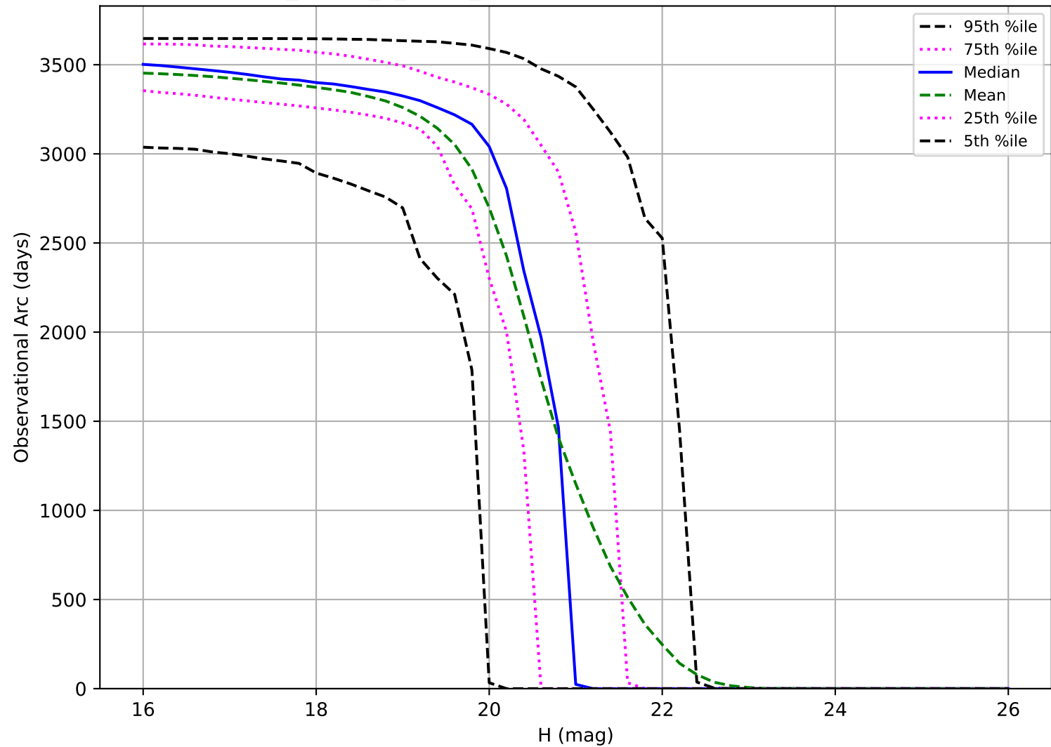
too_ignore_5_4v3.4_10yrs: Observational Arc Length MBA
