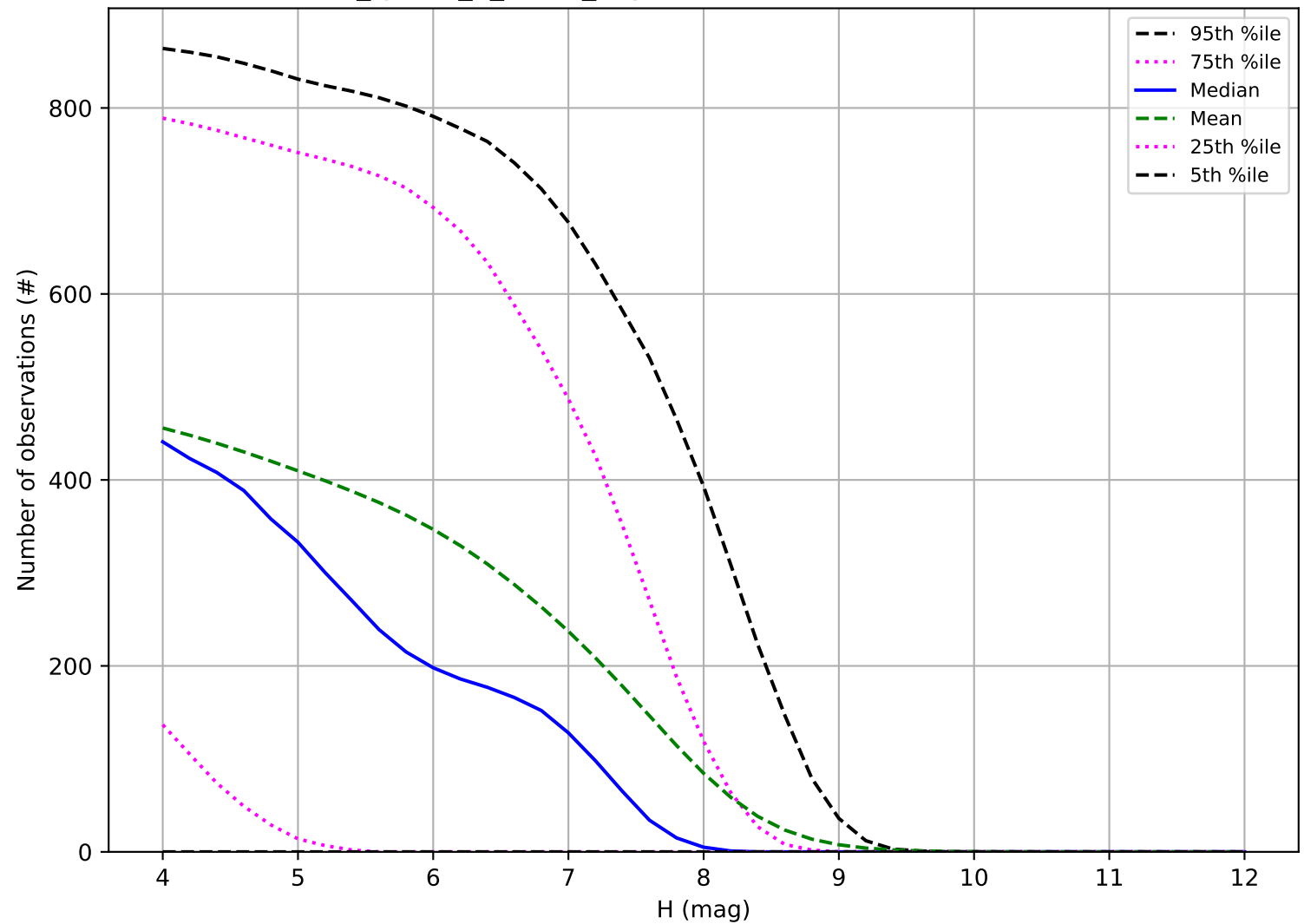
too_ignore_5_4v3.4_10yrs: Number of observations TNO
