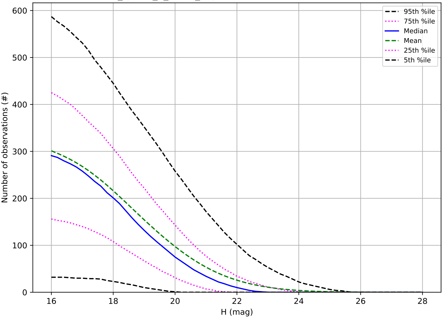
too_ignore_5_4v3.4_10yrs: Number of observations NEO
