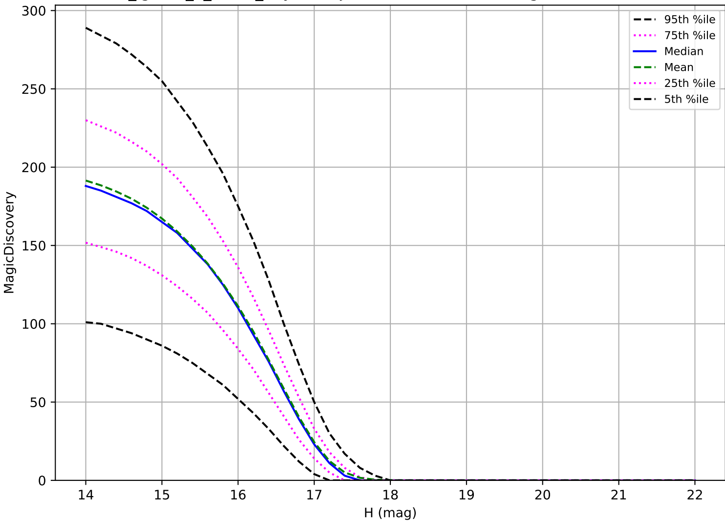
too_ignore_5_4v3.4_10yrs: Trojan 6 detections in 60 nights detection loss
