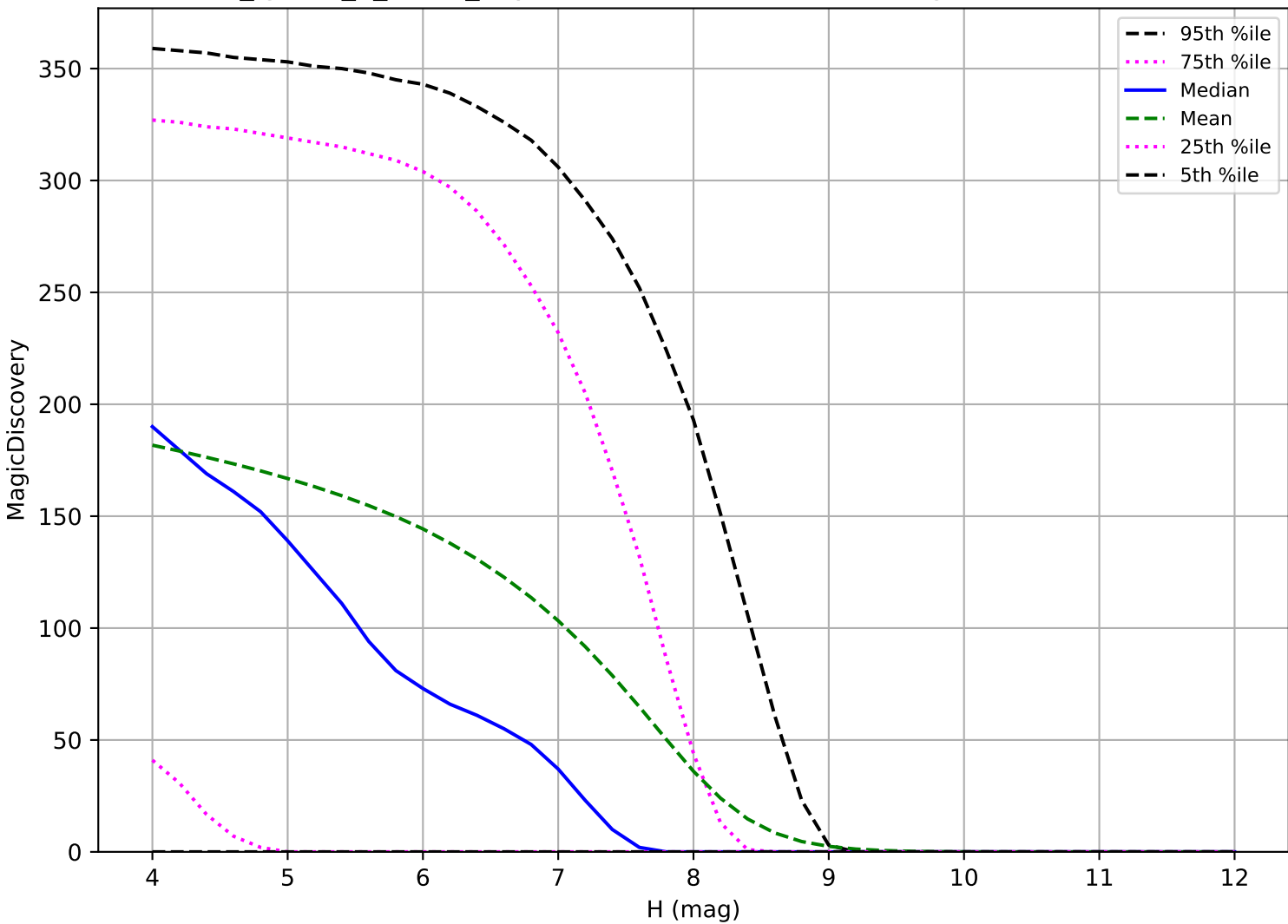
too_ignore_5_4v3.4_10yrs: TNO 6 detections in 60 nights detection loss
