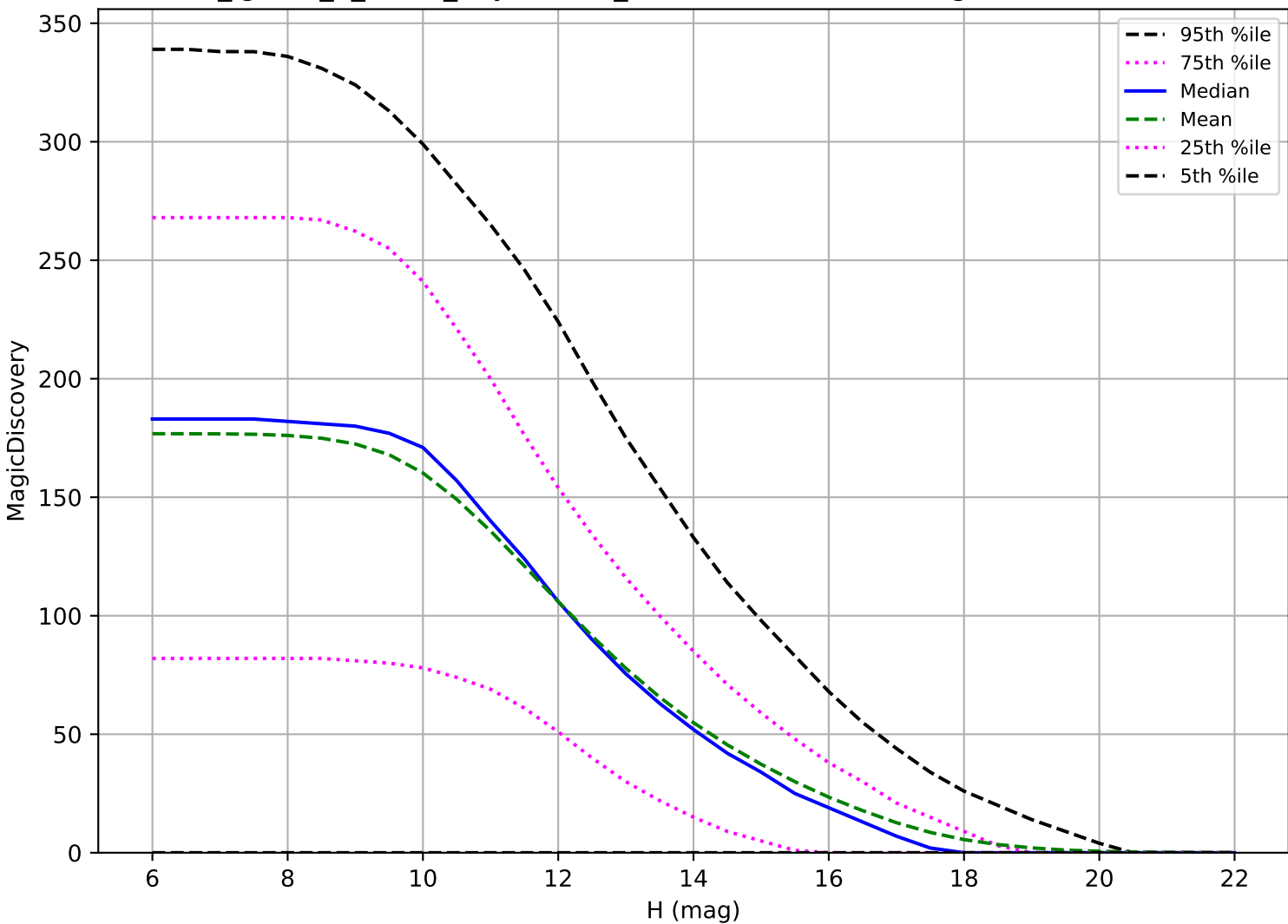
too_ignore_5_4v3.4_10yrs: OCC_r5 6 detections in 60 nights detection loss
