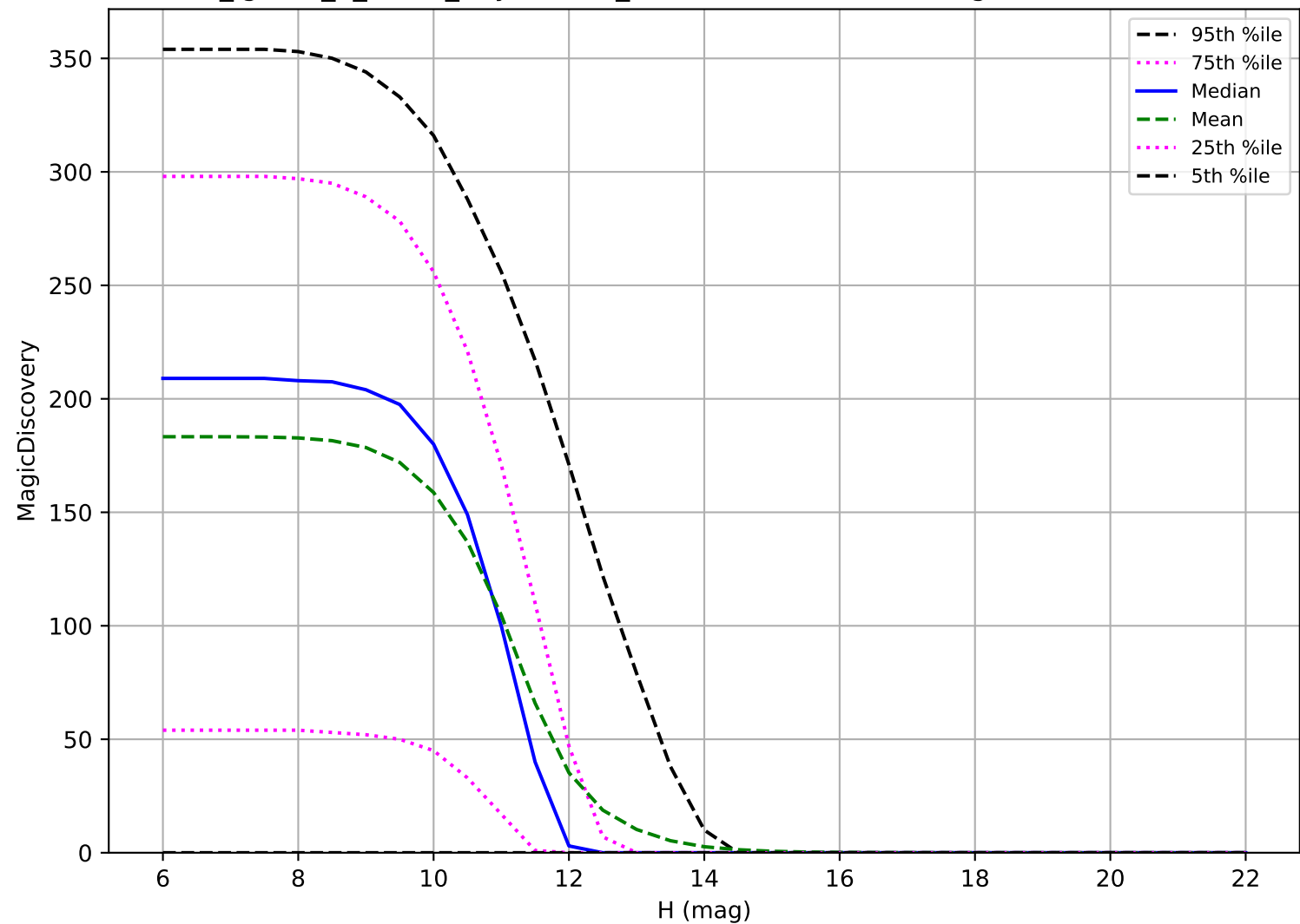
too_ignore_5_4v3.4_10yrs: OCC_r20 6 detections in 60 nights detection loss
