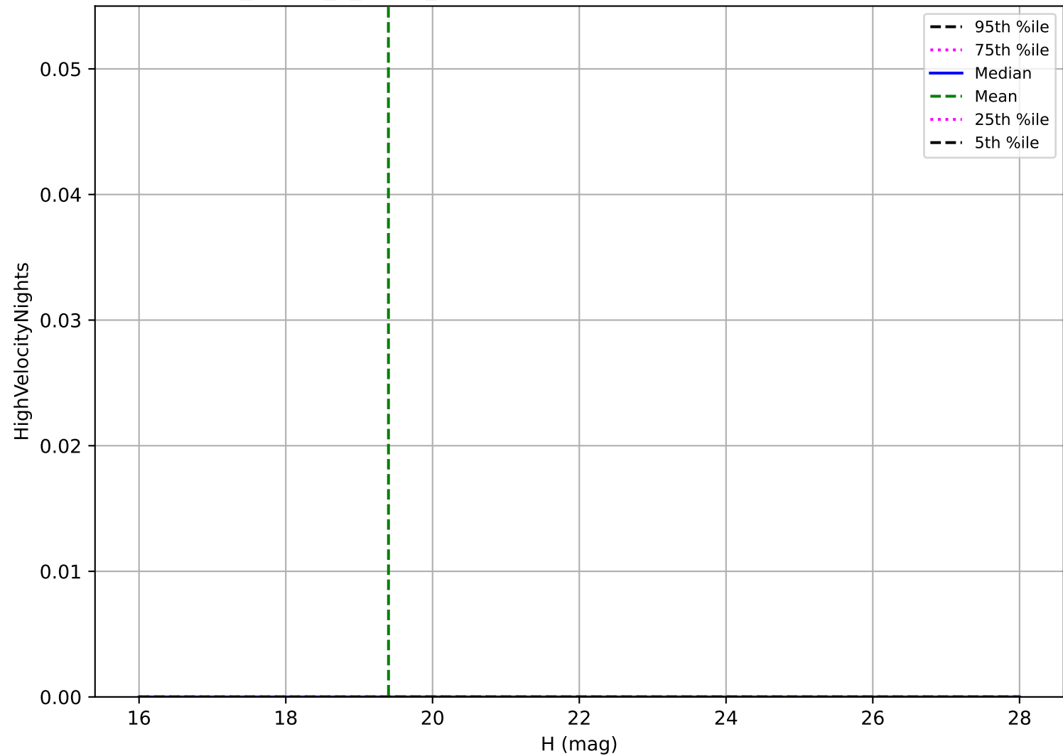
too_ignore_5_4v3.4_10yrs: Vatira High velocity pair detection loss
