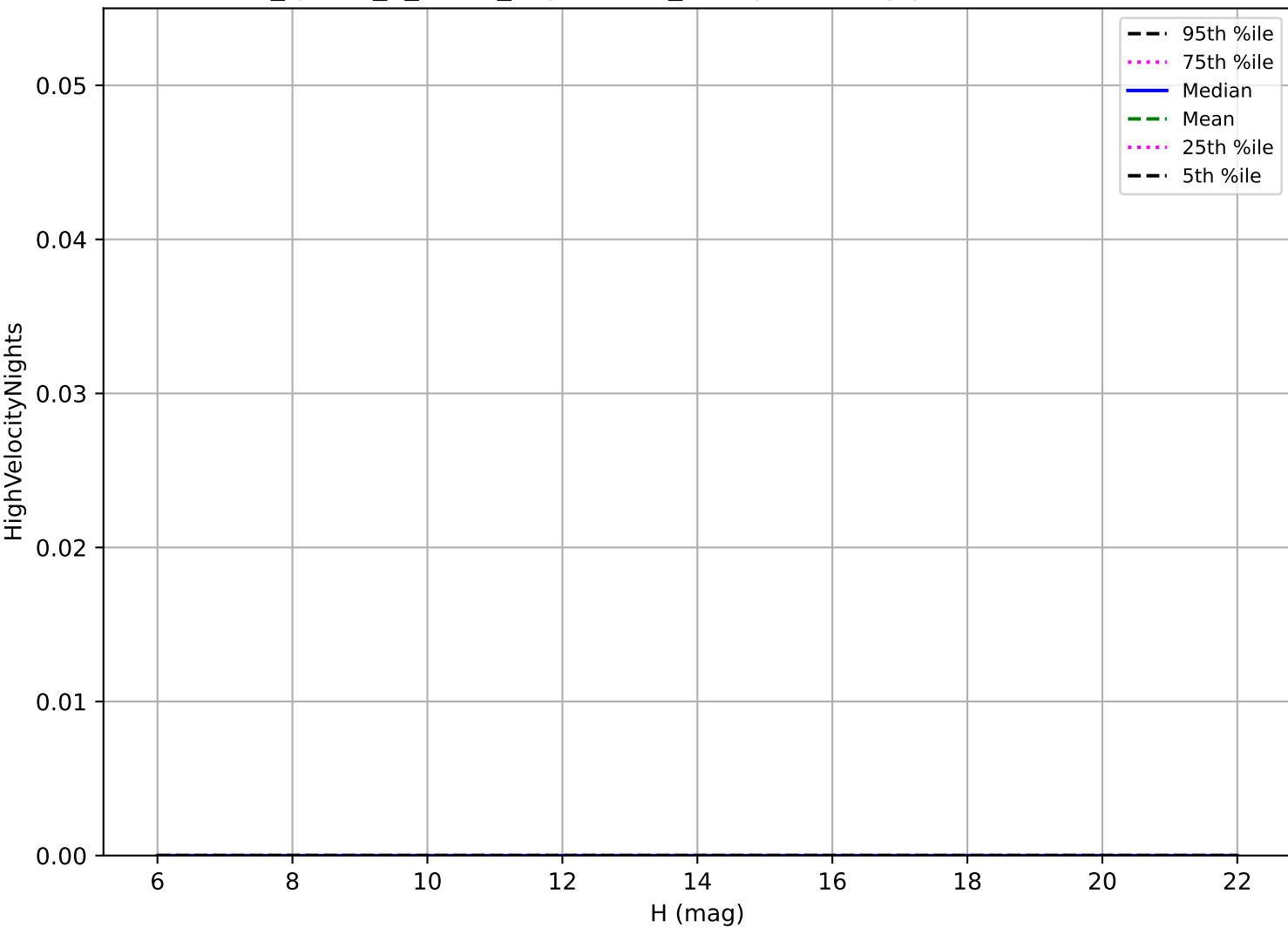
too_ignore_5_4v3.4_10yrs: OCC_r5 High velocity pair detection loss
