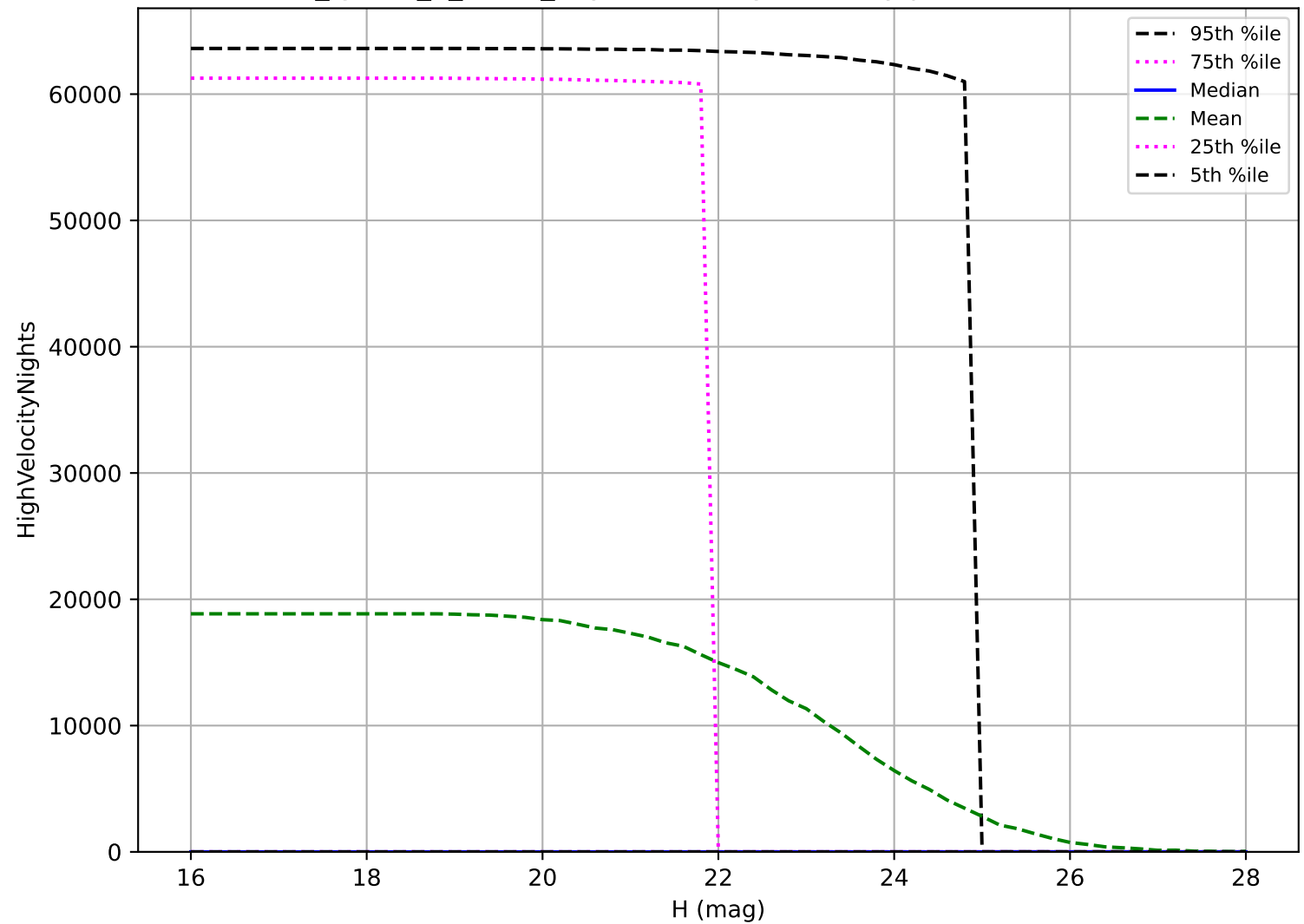
too_ignore_5_4v3.4_10yrs: NEO High velocity pair detection loss
