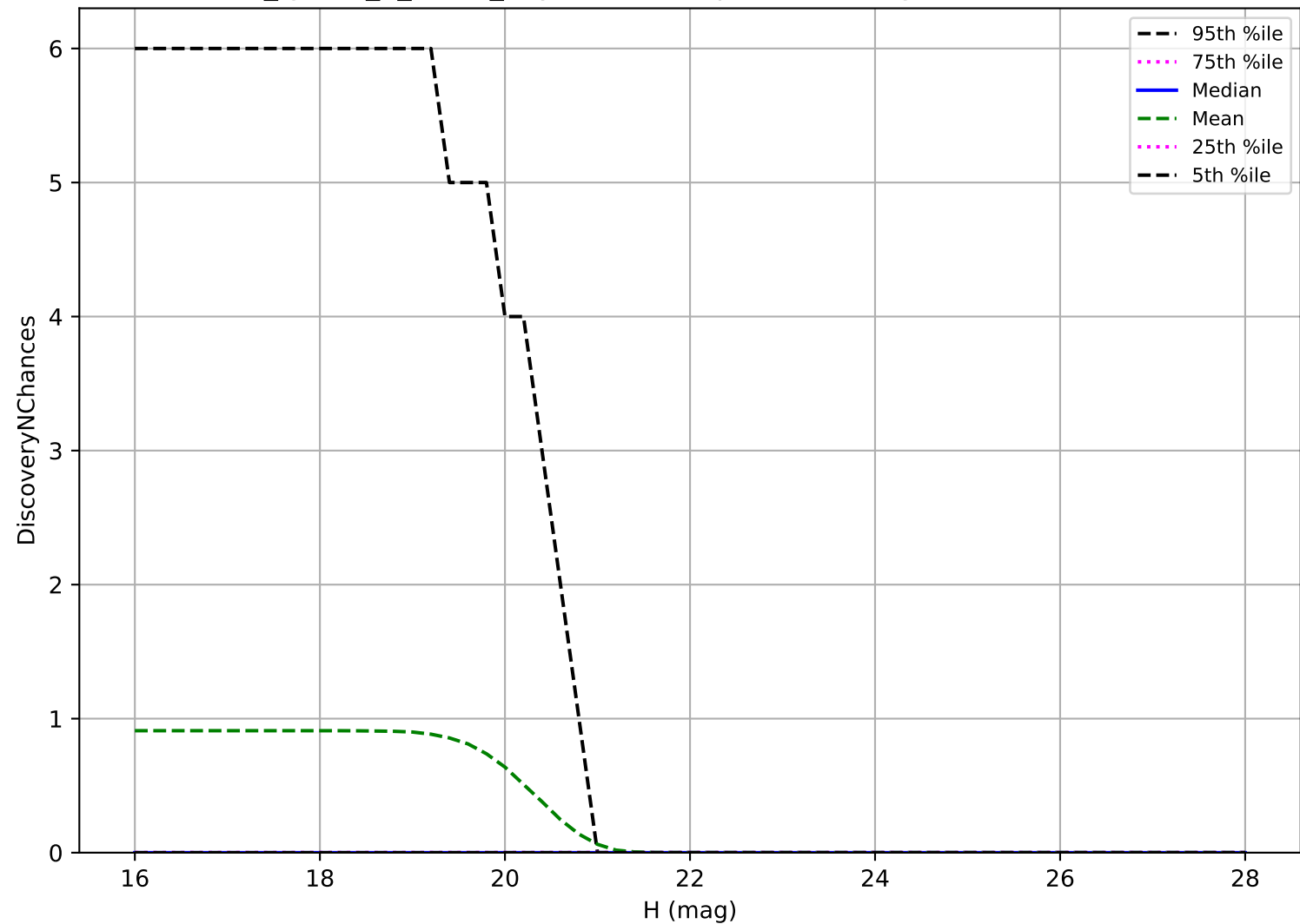
too_ignore_5_4v3.4_10yrs: Vatira 3 pairs in 15 nights detection loss
